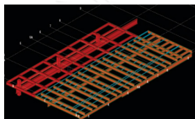
Chiller Supporting Structure
