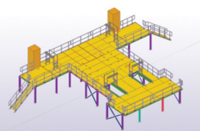
Conveyor Transfer Tower-2
