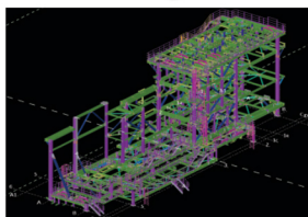
Oil & Gas Pipe Rack Structure
